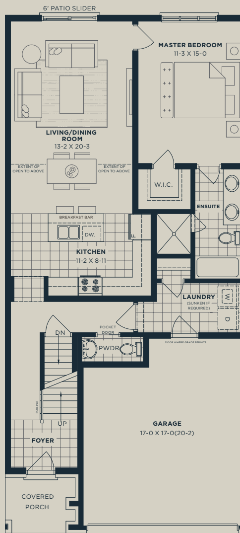
ELEVATION A LOFT FLOOR PLAN
